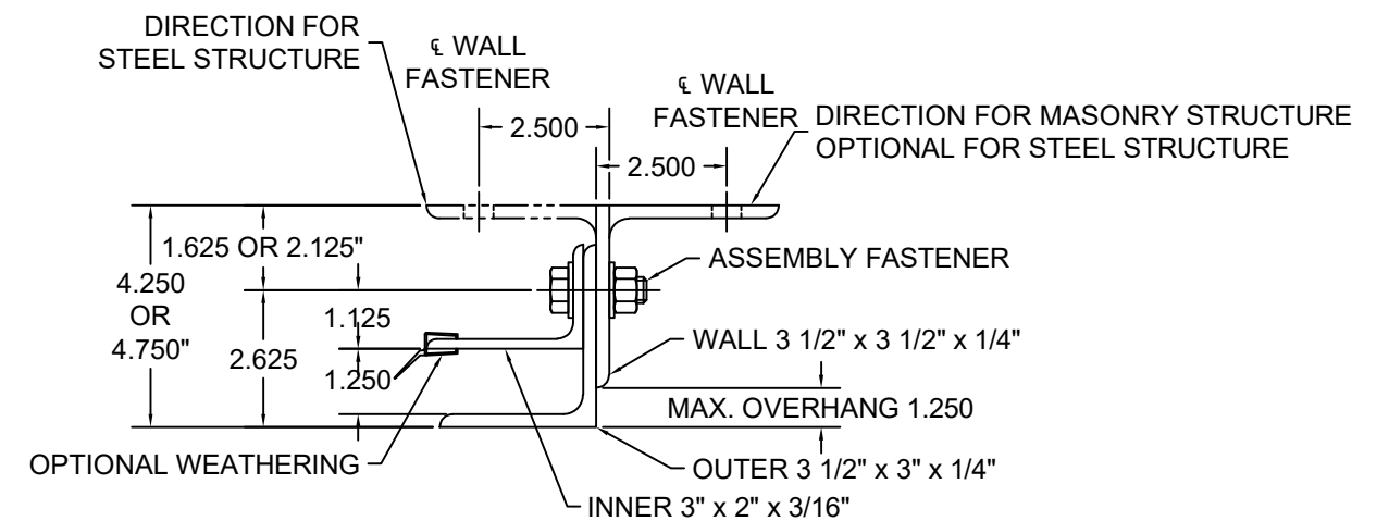
GUIDE ASSEMBLY TYPE 344* (NON-WINDLOCK) SCALE: 3" = 1'-0"
